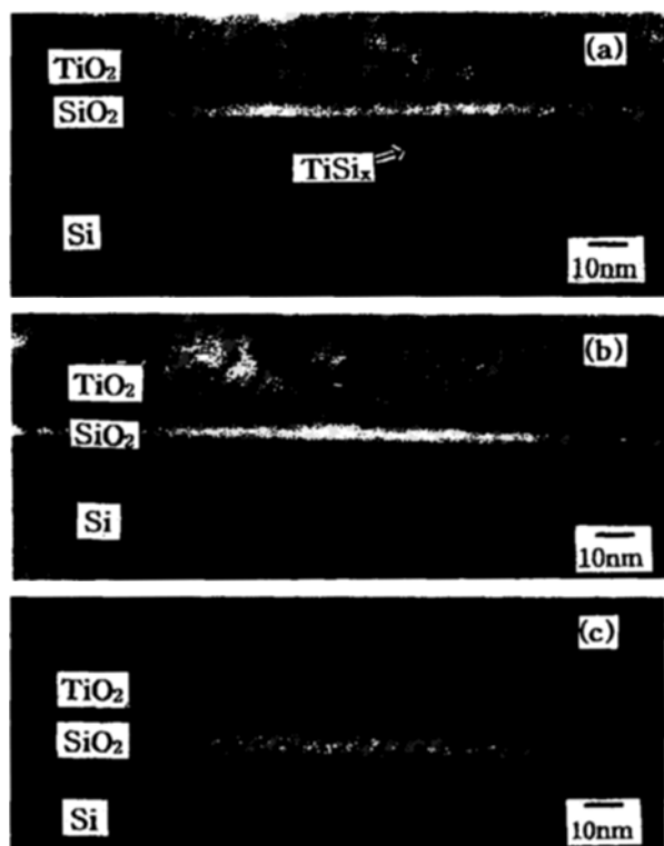
Fig. 9. TEM photographs of the \text{TiO}_2 films annealed: (a) \text{TiO}_2 on Si annealed at 800^\circ\text{C} for 60 s; (b) \text{TiO}_2 on \text{SiO}_2/\text{Si} annealed at 800^\circ\text{C} for 60 s; (c) \text{TiO}_2 on \text{SiO}_2/\text{Si} annealed at 1,000^\circ\text{C} for 1 h.
