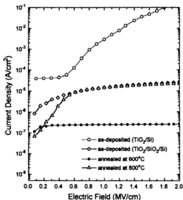
Fig. 7. Current density vs electric field curves for \text{TiO}_2 films on Si and \text{SiO}_2/\text{Si} substrates annealed at various temperatures for 60 s.
